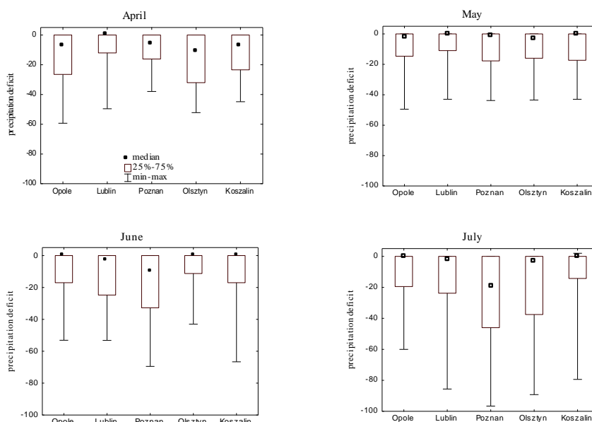
Fig. 2. Winter wheat precipitation deficiencies
