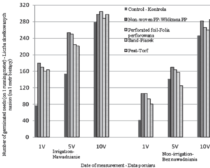
Fig. 1. The effect of stand improving methods on the emergence dynamic of garden dill ( Anethum graveolens L.) in 2009 and 2010
